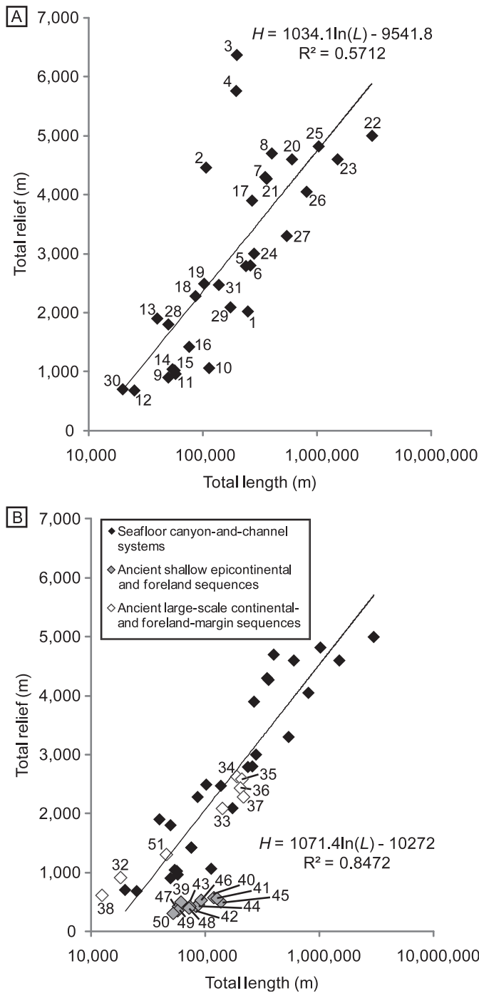
FIG. 4.— A ) Relief versus length of seafloor canyon-and-channel systems. Numbers correspond to systems in Table 1. B ) Relief versus length of seafloor canyon-and-channel systems except the San Antonio (2), Kushiro (3), and Aoga (4) systems. Ancient subsurface and outcropping paleo-shelf-slope-basin-floor sequences are also included (Table 2). Only seafloor data (black diamonds) were used in determining the correlation function.
